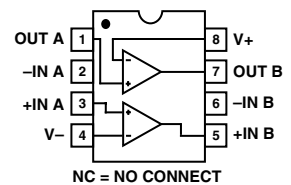
8-Lead HERMETIC DIP (Z-Suffix)
