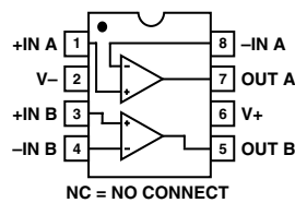
8-Lead SO (S-Suffix)
