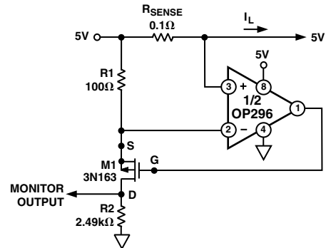
Figure 11. A High-Side Load Current Monitor
