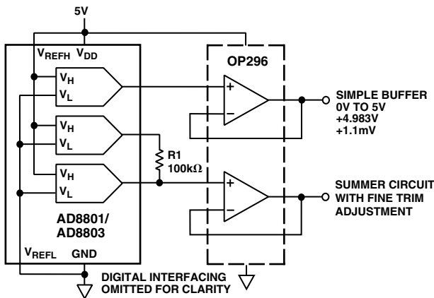
Figure 10. Buffering a TrimDAC Output
