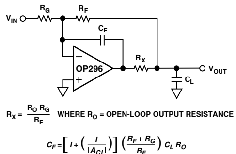
Figure 4. In-the-Loop Compensation Technique for Driving Capacitive Loads
