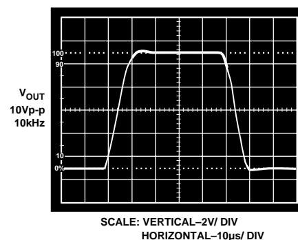
Figure 18. A 3-Pole, 40 kHz Low-Pass Filter
