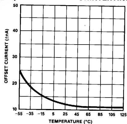
MATCHING CHARACTERISTIC; AVERAGE OFFSET CURRENT vs TEMPERATURE (INVERTING OR NONINVERTING)
