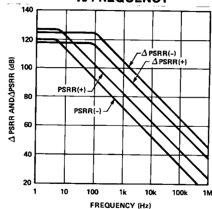
PSRR AND ΔPSRR vs FREQUENCY
