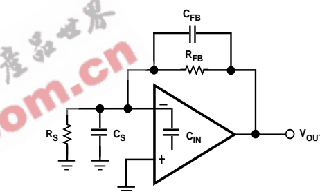
Figure 14. Compensating the Feedback Pole
