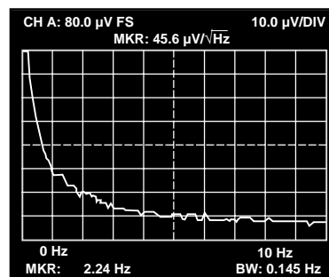
Figure 6. 1/f Noise Corner, V_S = ±15 V, A_V = 1000
