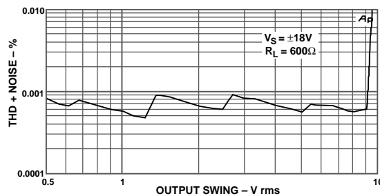
Figure 4. Headroom, THD + Noise vs. Output Amplitude (V rms); R_{LOAD} = 600 Ω, V_{SUP} = ±18 V
