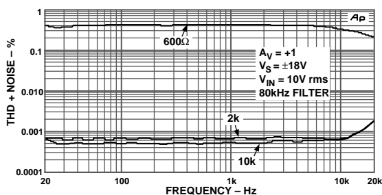
Figure 3. THD + Noise vs. R_{LOAD} ; V_{IN} = 10 V rms, ±18 V Supplies
