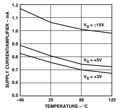
Figure 10. Supply Current vs. Temperature
