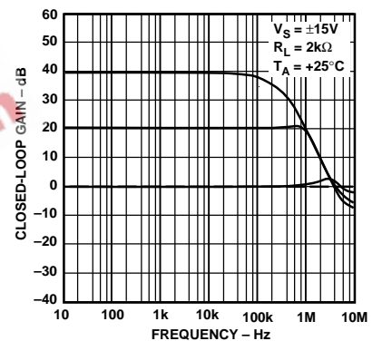
Figure 18. Closed-Loop Gain vs. Frequency (2 kΩ Load)
