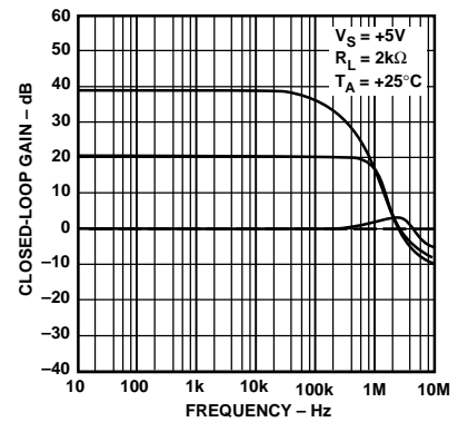
Figure 17. Closed-Loop Gain vs. Frequency (2 kΩ Load)
