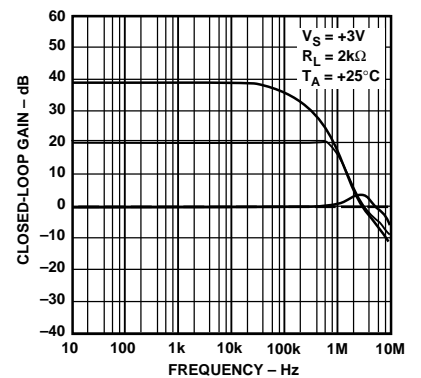
Figure 19. Closed-Loop Gain vs. Frequency (2 kΩ Load)
