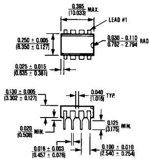
8 Lead Plastic DIP \theta_{JA} = 120^{\circ}\text{C/W} \theta_{JC} = 70^{\circ}\text{C/W}
