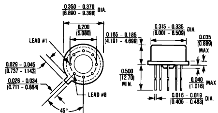
8 Lead T0-99 \theta_{JA} = 150^{\circ}\text{C/W} \theta_{JC} = 45^{\circ}\text{C/W}
