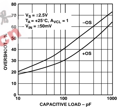
Figure 27. Small Signal Overshoot vs. Capacitive Load
