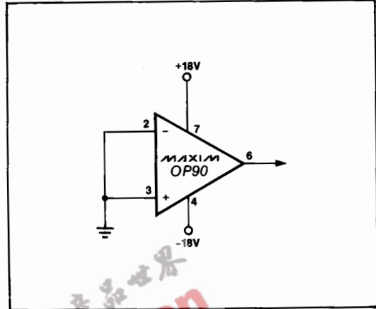
Figure 2. Burn-In Circuit
