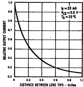
Coupling Characteristics of OP161SL and OP501SL
