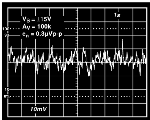
FIGURE 32. 0.1 Hz TO 10 Hz NOISE
