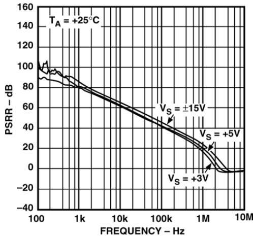
FIGURE 25. PSRR VS. FREQUENCY
