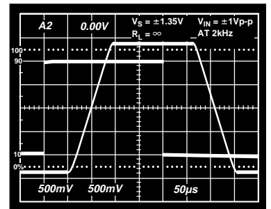
Figure 30. Saturation Recovery Time
