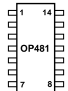
14-Lead TSSOP (RU Suffix)
