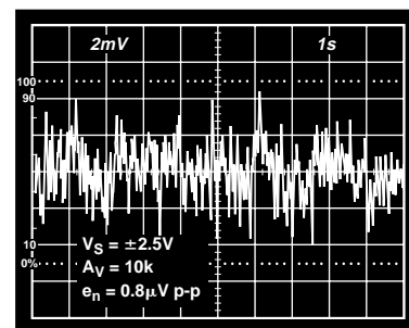
Figure 30. 0.1 Hz to 10 Hz Noise
