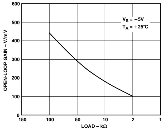
Figure 19. Open Loop Gain vs. Resistive Load
