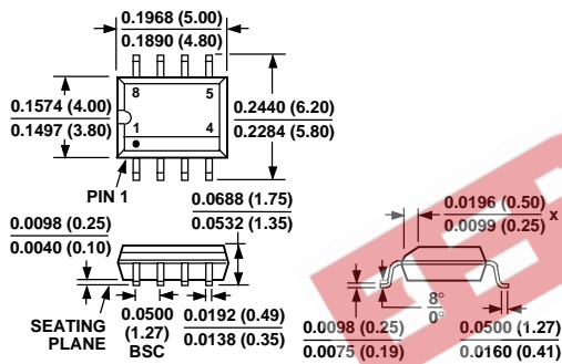
8-Lead Narrow Body SOIC (SO-8)
