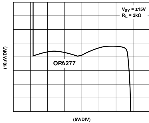
Figure 52. Gain Linearity
