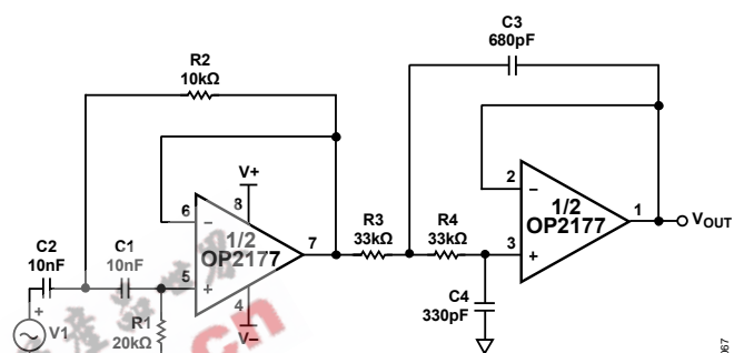
Figure 67. Two-Stage, Band-Pass KRC Filter
