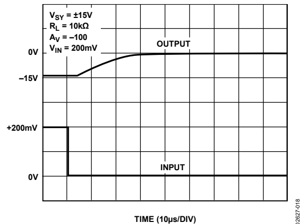
Figure 18. Positive Overtolerance Recovery
