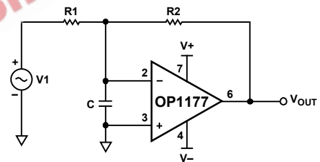
Figure 61. EMI Reduction
