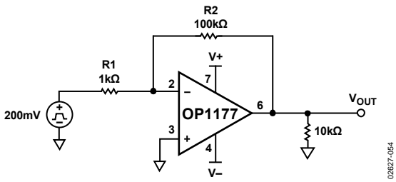
Figure 54. Test Circuit for Overload Recovery Time
