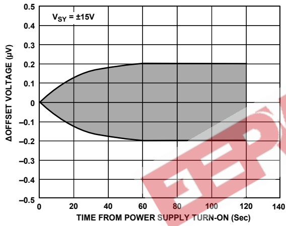
Figure 26. Warm-Up Drift
