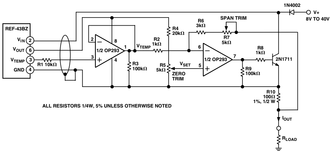
Figure 11. Temperature to 4–20 mA Transmitter
