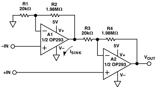
Figure 9. A Conventional Instrumentation Amplifier
