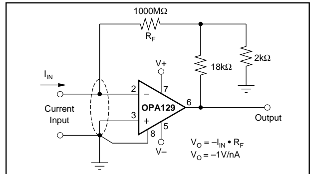
FIGURE 4. Current-to-Voltage Converter.
