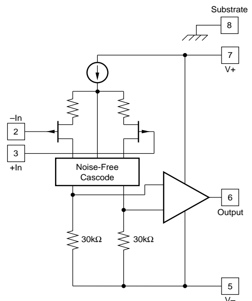
Simplified Circuit
