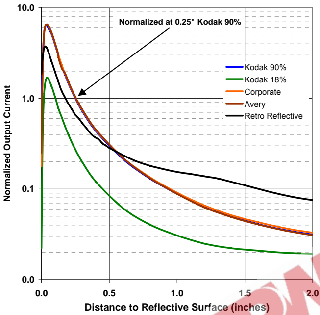
OPB730 - Normalized Collector Current vs. Object Distance
