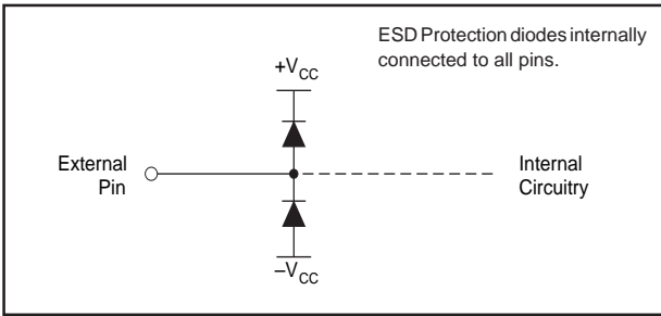
FIGURE 3. Internal ESD Protection.
