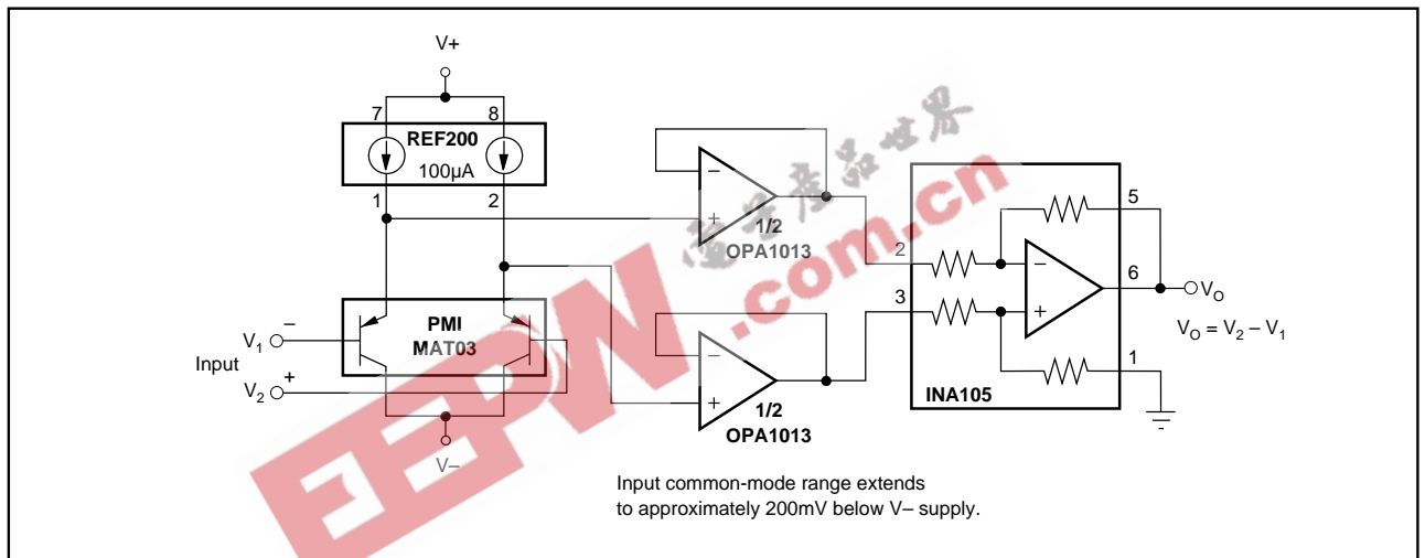
FIGURE 3. Instrumentation Amplifier.
