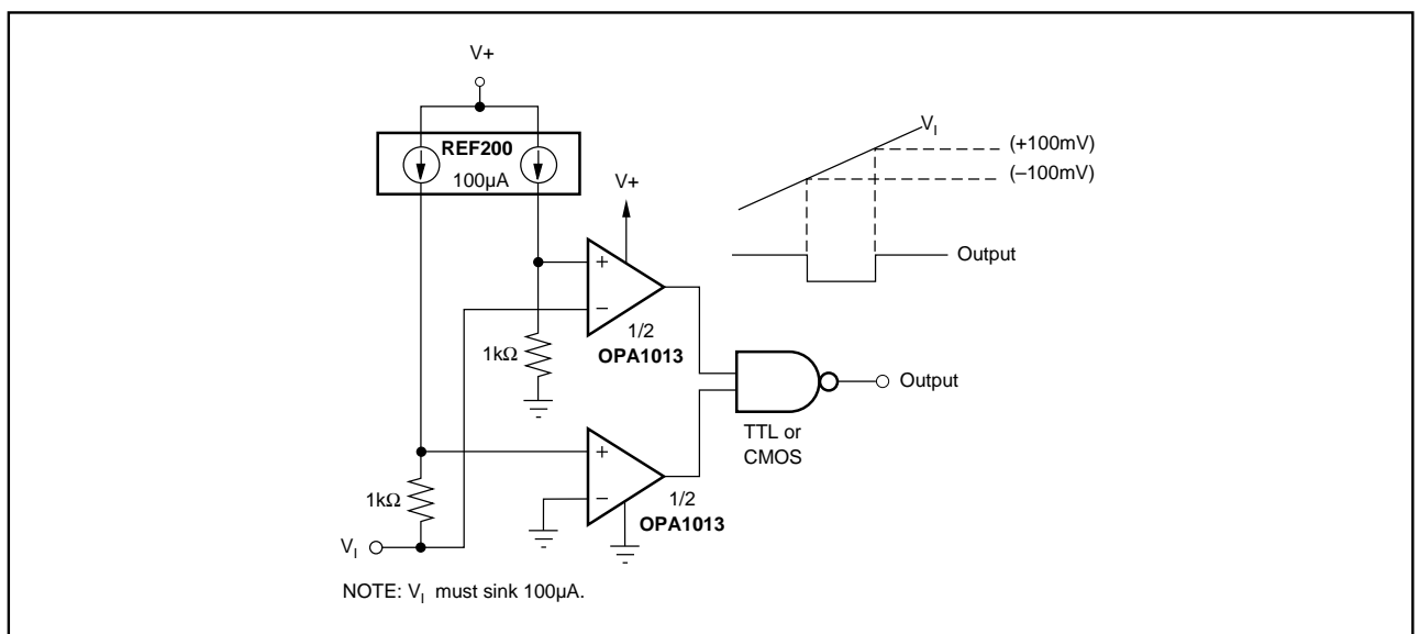
FIGURE 4. Window Comparator.
