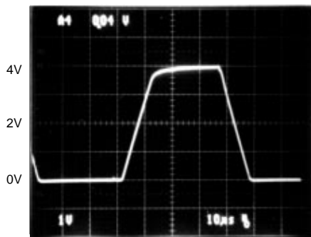
LARGE SIGNAL TRANSIENT RESPONSE V_S = 5V/0V, G = +1, \text{No Load}
