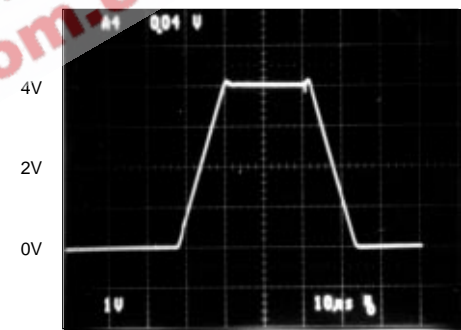
LARGE SIGNAL TRANSIENT RESPONSE V_S = 5V/0V, G = +1, R_L = 4.7k\Omega to 5V
