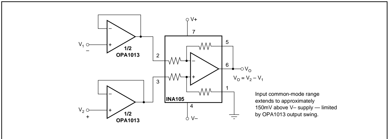
FIGURE 2. Instrumentation Amplifier.
