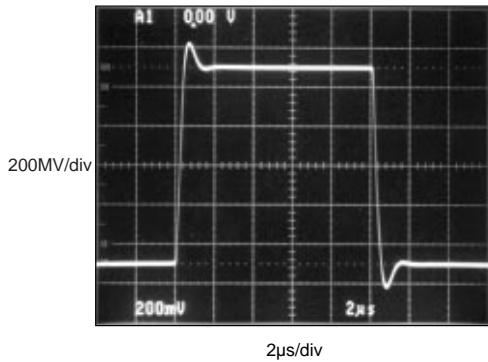
SMALL SIGNAL RESPONSE G = 3 , C_L = 1nF
