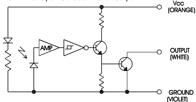
OPB716: Open-Collector Buffer Output
