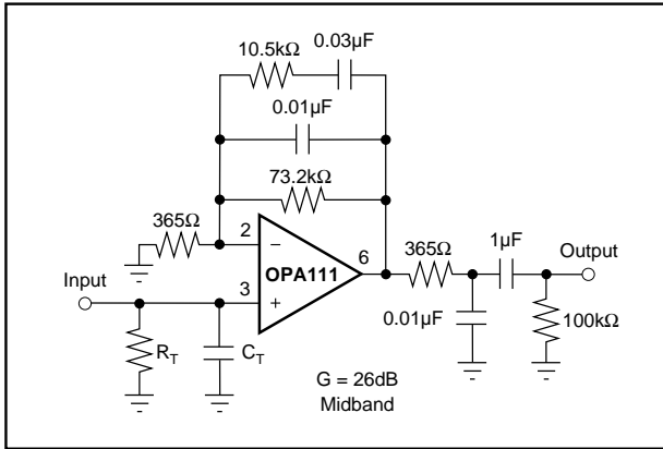
FIGURE 14. RIAA Equalized Phono Preampfier.
