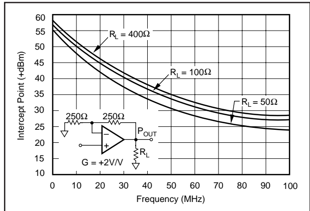
FIGURE 9. Two-Tone Third-Order Intermodulation Intercept vs Frequency.
