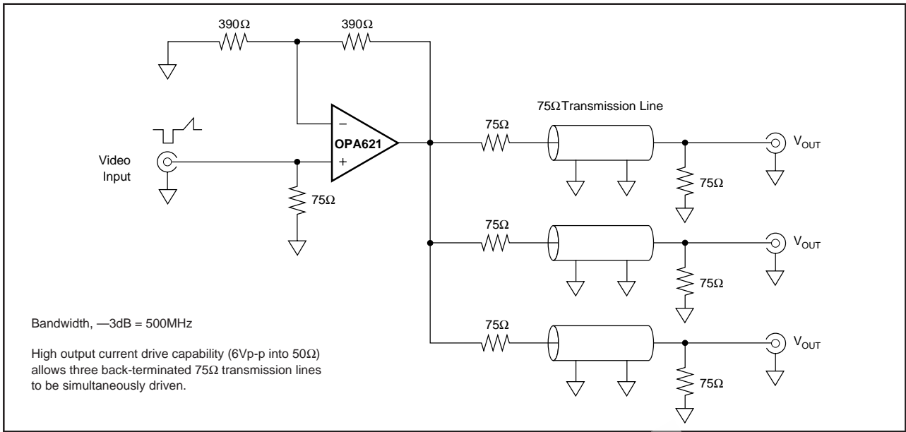
FIGURE 15. Video Distribution Amplifier.
