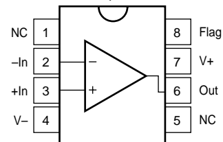
DIP-8 (P)
