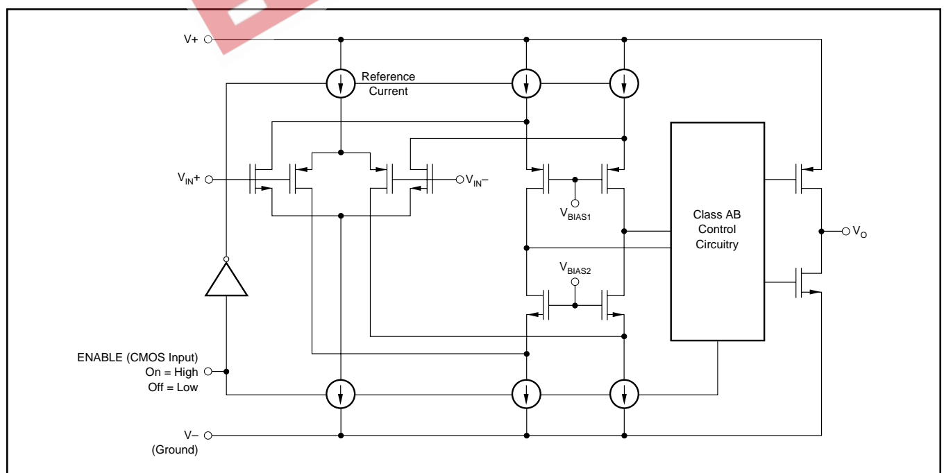
FIGURE 2. Simplified Schematic.
