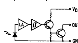
OPL551-OC (Open-Collector Output) Inverter
