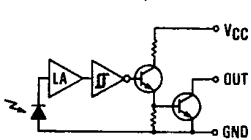
OPL550-OC (Open-Collector Output) Buffer
