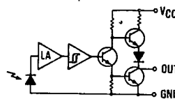
OPL551 (Totem-Pole Output) Inverter
