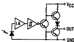
OPL550 (Totem-Pole Output) Buffer
