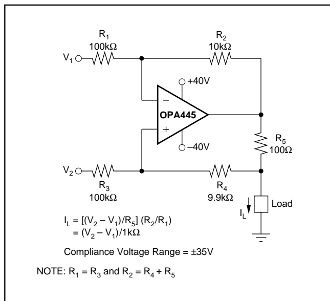
FIGURE 9. Voltage-to-Current Converter.
