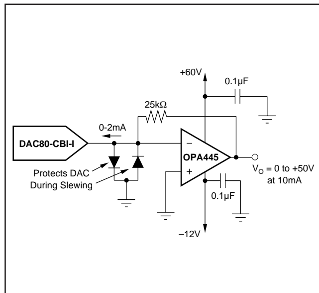
FIGURE 10. Programmable Voltage Source.
