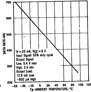
Data Rate vs Ambient Temperature
