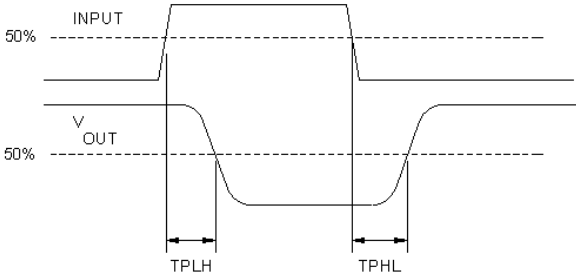
Figure 2: Input/Output Waveforms
