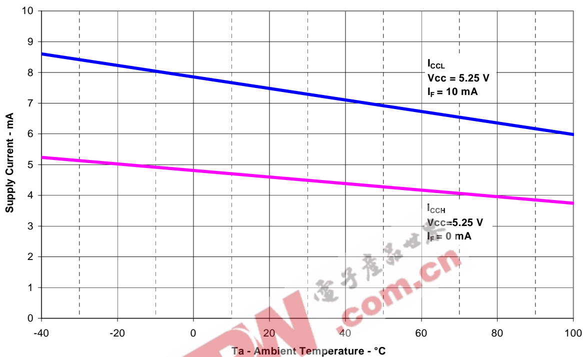
I_{CCH} & I_{CCL} vs. Ambient Temperature
