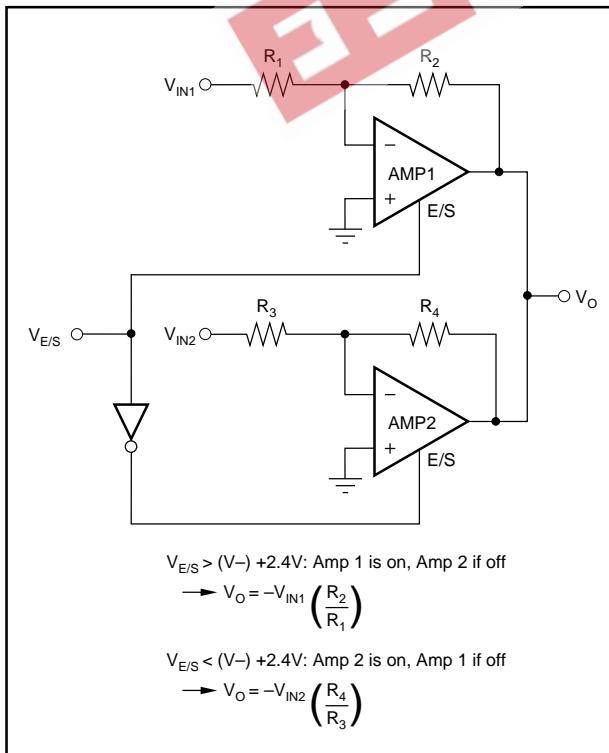
FIGURE 15. Swap Amplifier.
