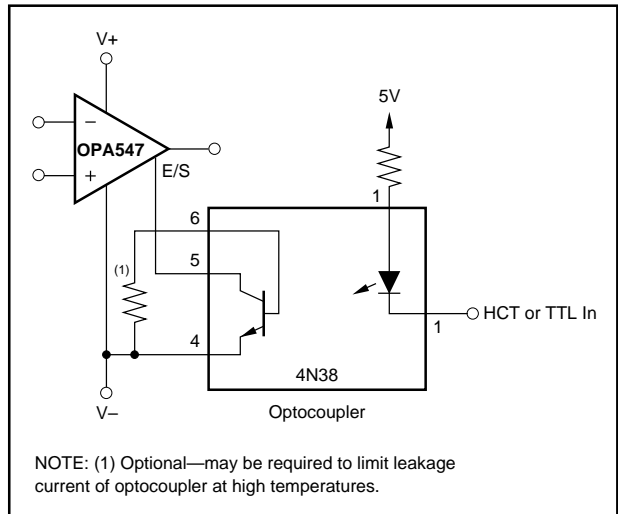
FIGURE 6. Output Disable with Dual Supplies.
