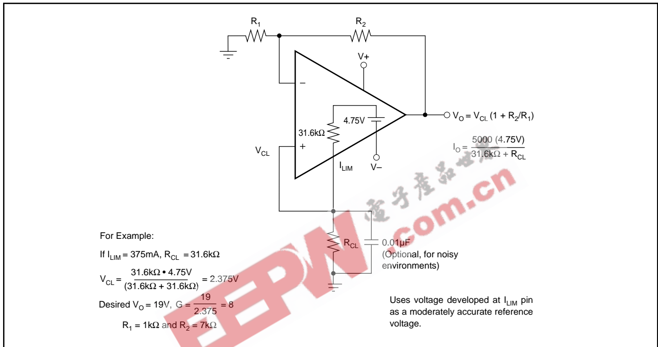
FIGURE 12. Voltage Source.
