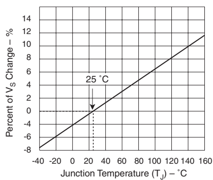
Normalized V_S Change versus Junction Temperature
