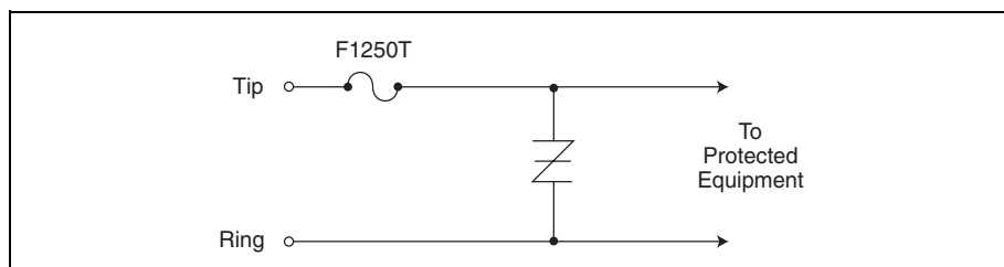
Figure 4.17 Metallic-only Solution using Teccor's "SB" or "EB" Series
