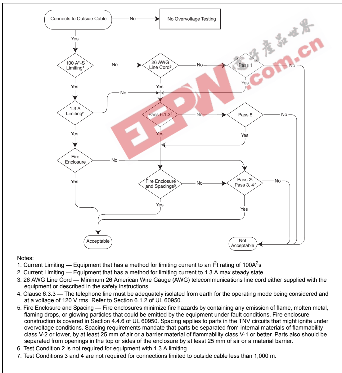
Figure 4.5 Overvoltage Flowchart
