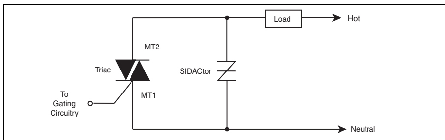
Figure 3.41 TRIAC Protection
