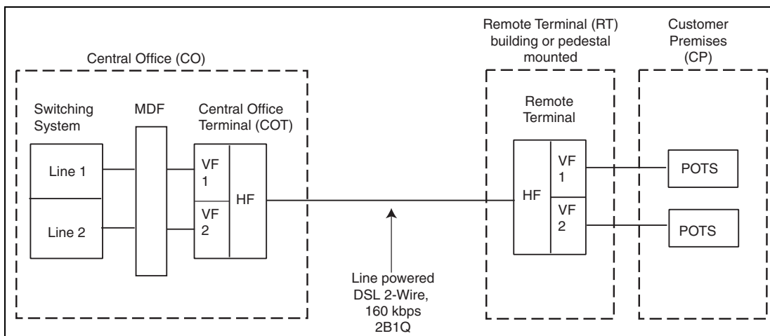
Figure 3.13 Pair Gain Overview
