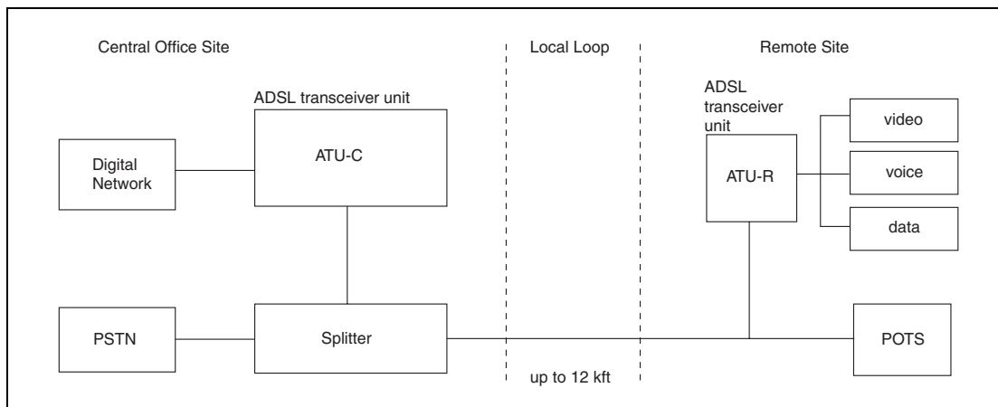
Figure 3.7 ADSL Overview
