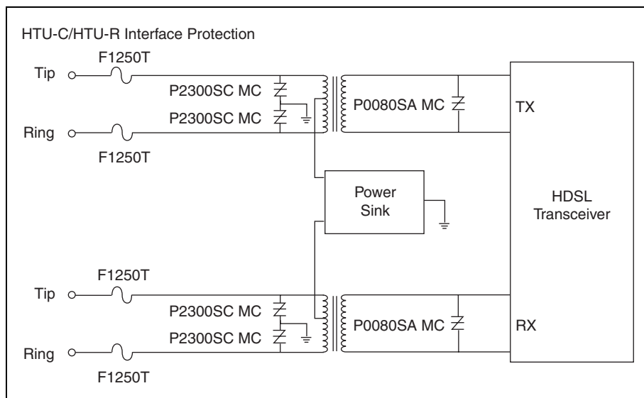
Figure 3.10 HDSL Protection
