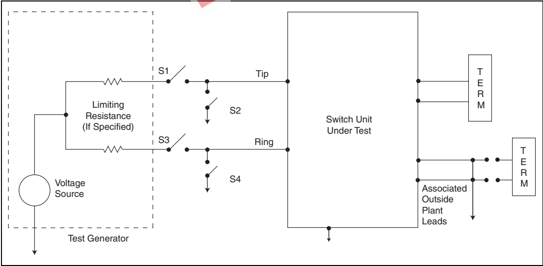
Figure 4.1 Connection Appearances
