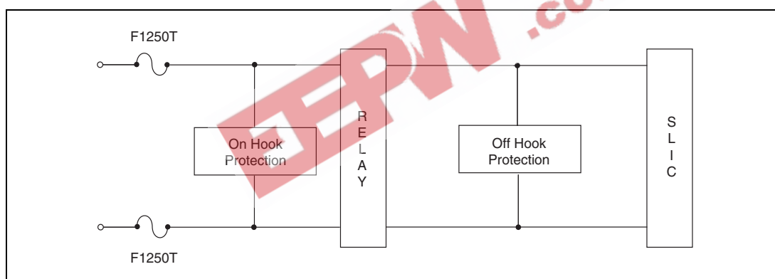
Figure 3.20 SLIC Overview
