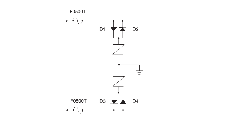
Figure 3.44 10Base-T Metallic and Longitudinal Protection
