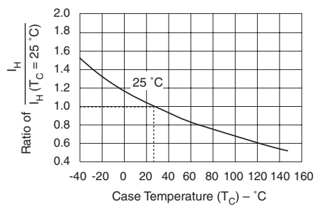
Normalized DC Holding Current versus Case Temperature
