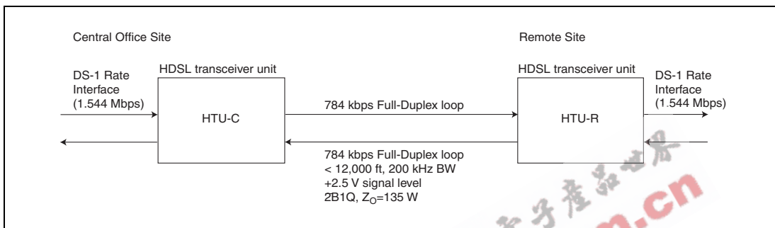
Figure 3.9 HDSL Overview
