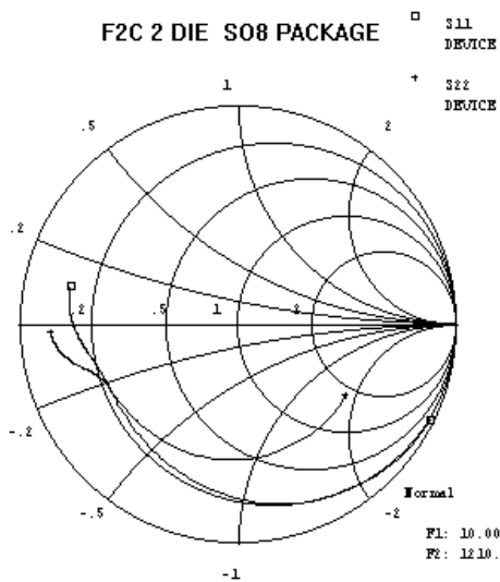
S11 & S22 SMITH CHART
