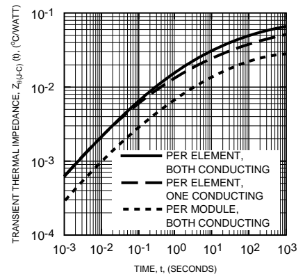
TRANSIENT THERMAL IMPEDANCE CHARACTERISTICS (JUNCTION-TO-CASE) Z JA
