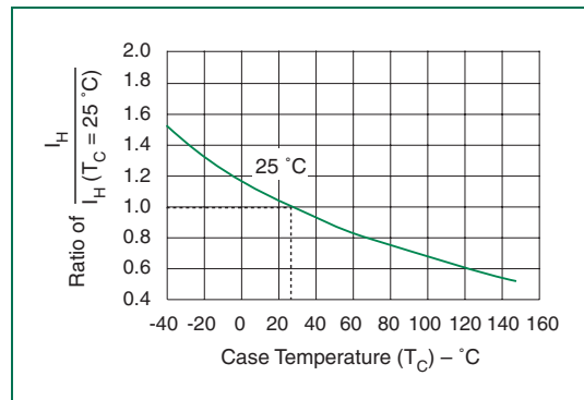
Normalized DC Holding Current versus Case Temperature
