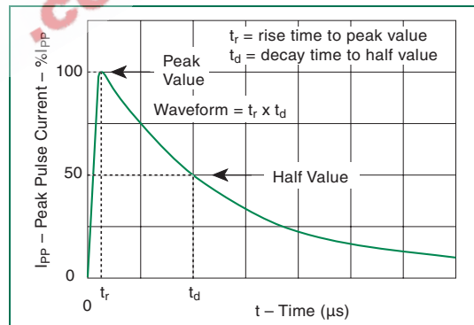
t_r \times t_d Pulse Waveform
