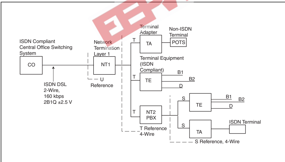
Figure 3.11 ISDN Overview
