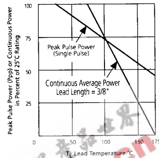
FIGURE 1 Derating Curve
