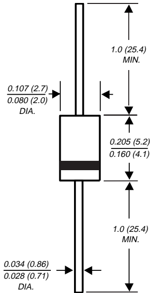
DO-204AL
