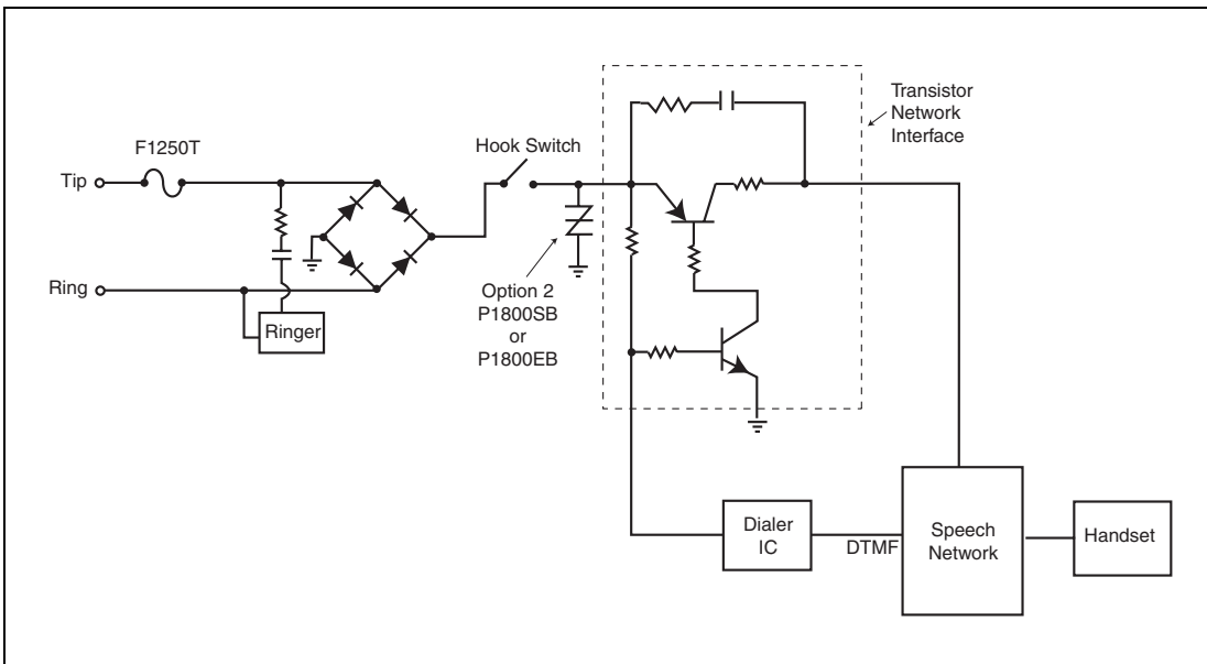
Figure 3.5 CPE Transistor Network Interface — Option 2
