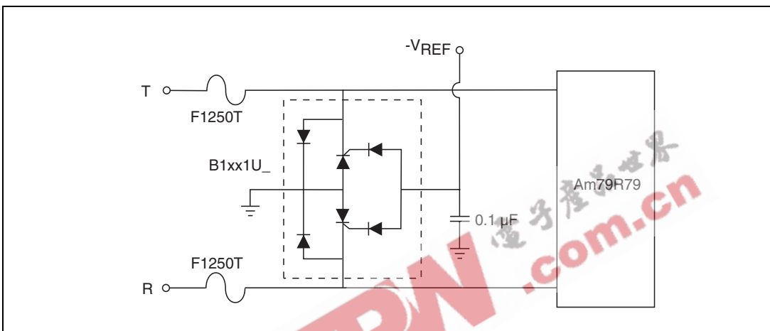
Figure 3.27 SLIC Protection with a Dual Batrax Device
