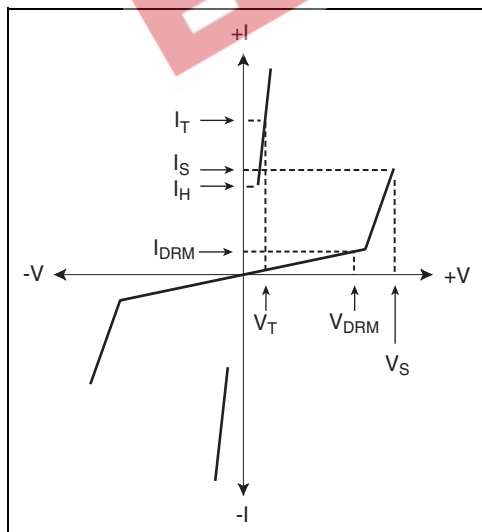
Figure 5.1 V-I Characteristics
