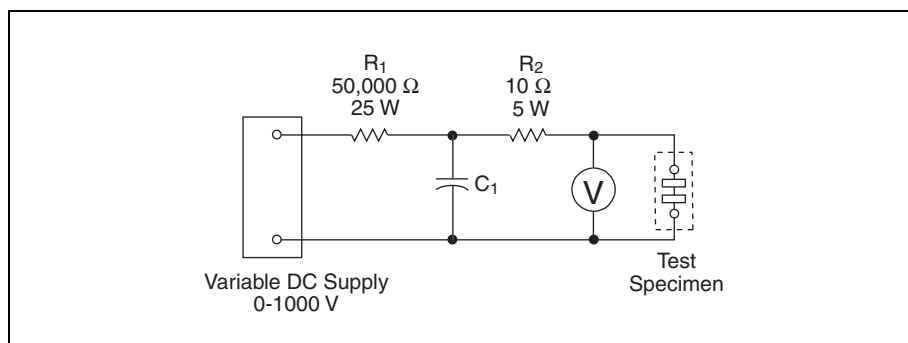
Figure 4.8 UL 497 Breakdown Voltage Measurement
