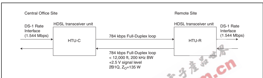
Figure 3.9 HDSL Overview
