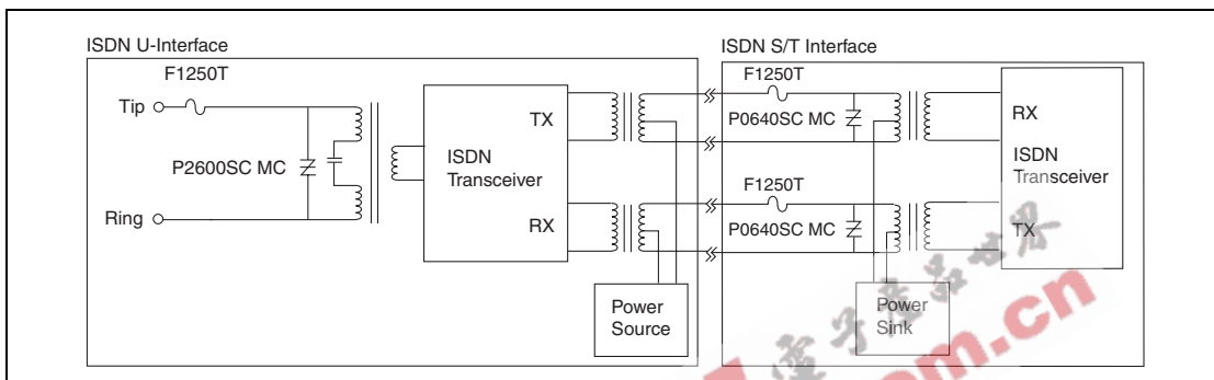
Figure 3.12 ISDN Protection
