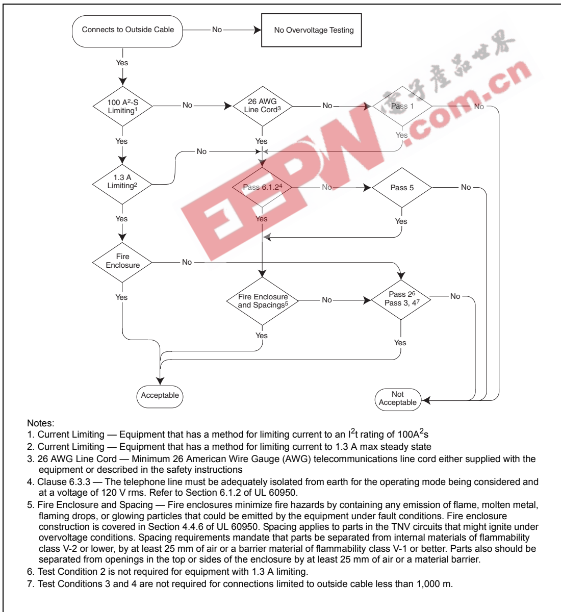
Figure 4.5 Overvoltage Flowchart
