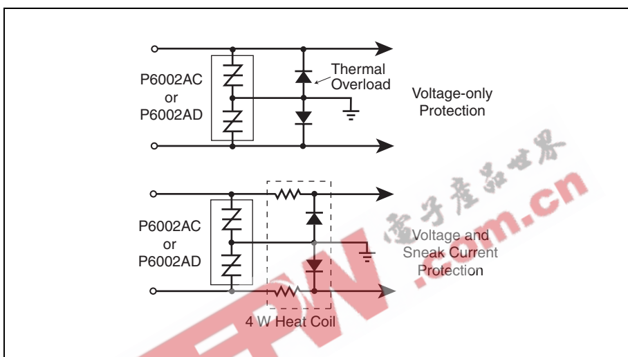
Figure 3.36 Primary Protection
