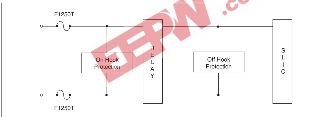
Figure 3.20 SLIC Overview
