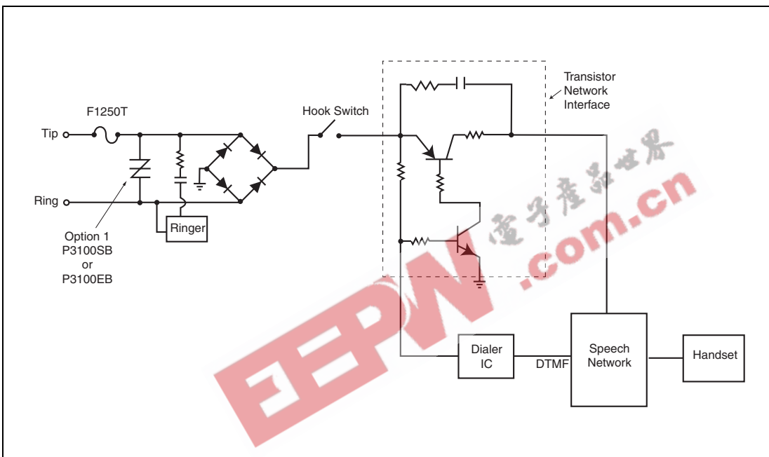
Figure 3.4 CPE Transistor Network Interface — Option 1
