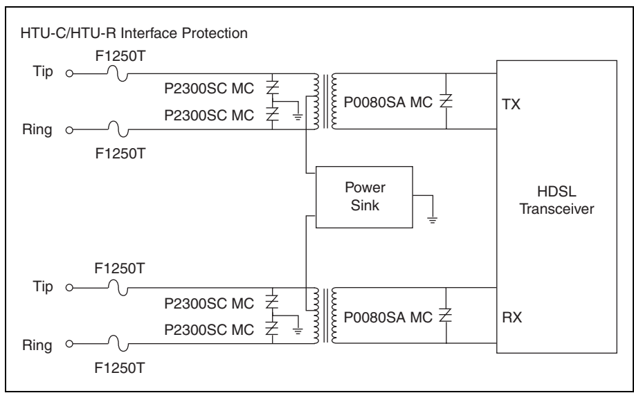
Figure 3.10 HDSL Protection
