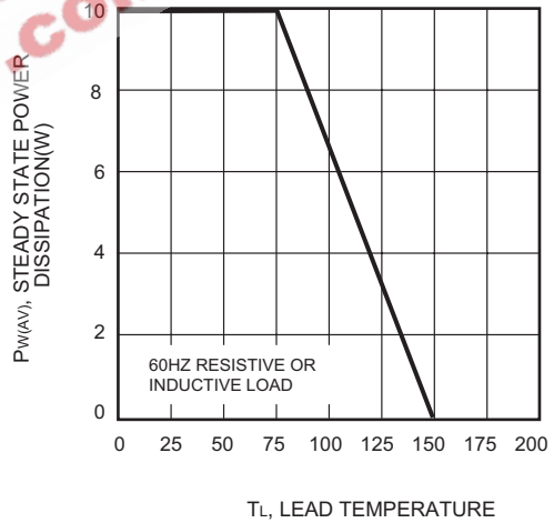
FIG.4 - STEADY STATE POWER DERATING CURVE
