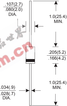
DO-41
