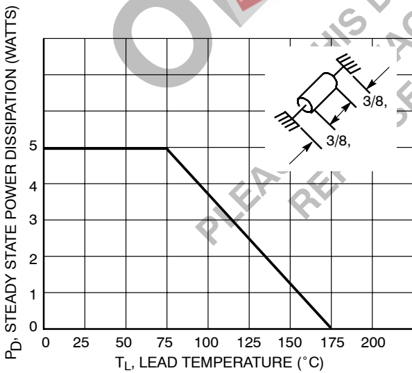
Figure 4. Steady State Power Derating
