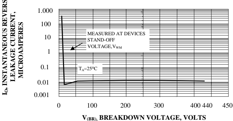
FIG. 7 - TYPICAL REVERSE LEAKAGE CHARACTERISTICS
