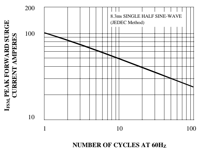
FIG. 6 - MAXIMUM NON-REPETITIVE FORWARD SURGE CURRENT UNIDIRECTIONAL
