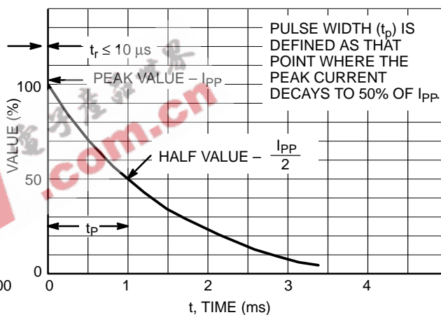
Figure 4. Pulse Waveform
