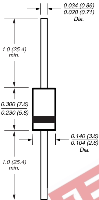
DO-204AC (DO-15)
