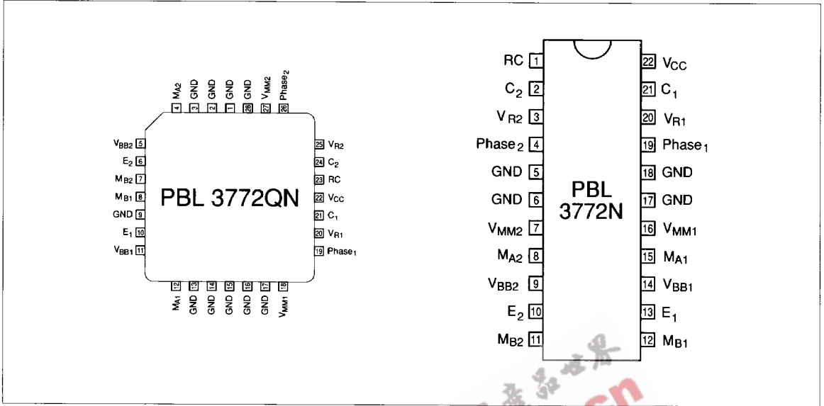
Figure 4. Pin configuration.
