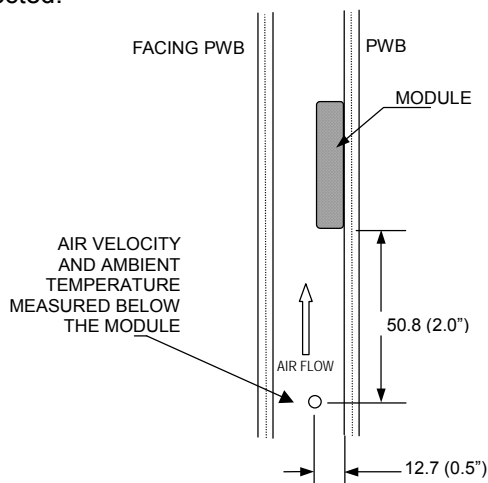
Note: Wind Tunnel Test Setup Figure Dimensions are in millimeters and (Inche) Figure 26: Wind tunnel test setup figure
