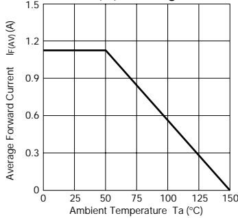
Ta—IF(AV) Derating
