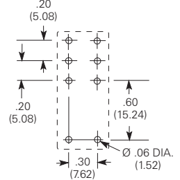
PC Board Layout (Bottom View)
