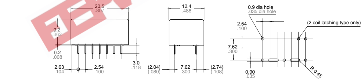
PC board pattern (Bottom view)
