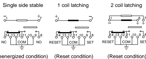
Schematic (Bottom view)
