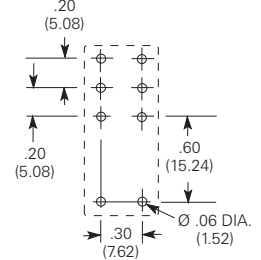
PC Board Layout (Bottom View)
